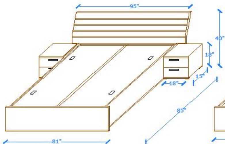
EXTERNAL VIEW
