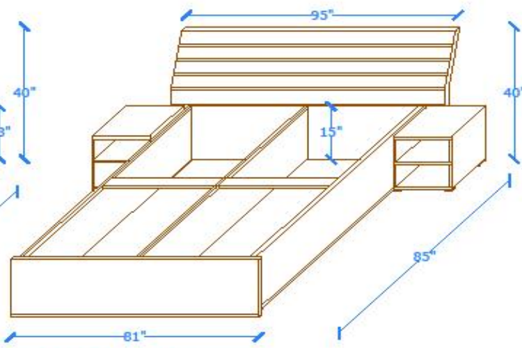
INTERNAL VIEW
