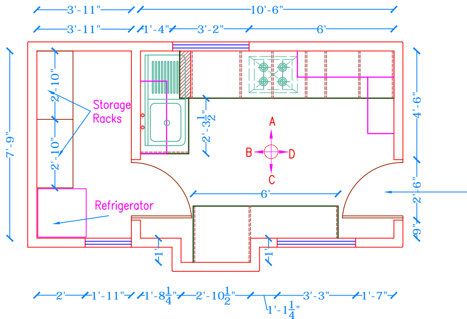
Kitchen Plan
