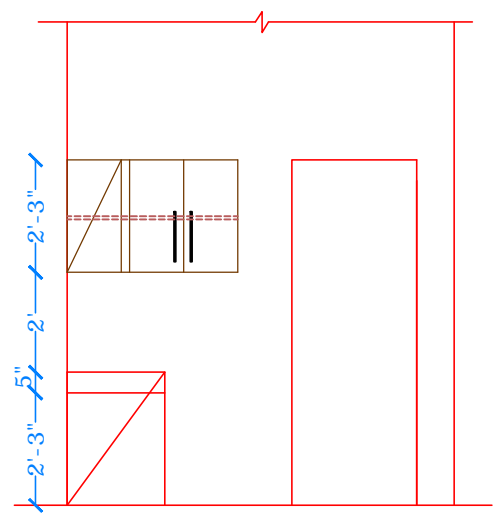
ELEVATION "D"
