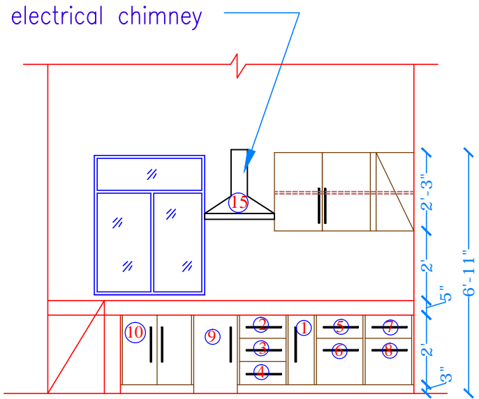
ELEVATION "A"
