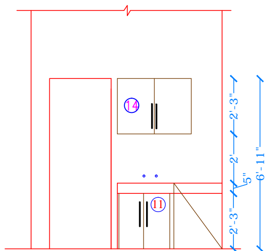
ELEVATION "B"
